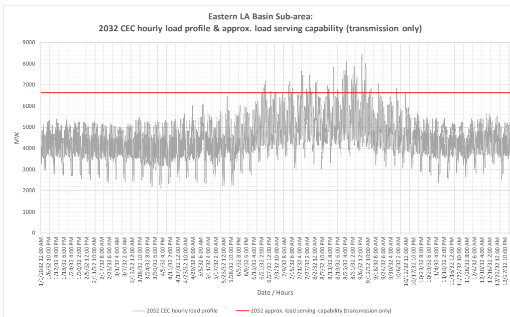
Figure J.3.2-79 Eastern LA Basin LCR Sub-area 2032 Forecast Hourly Profiles
