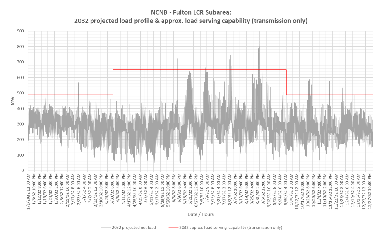
Figure J.3.2-12 Fulton LCR Sub-area 2032 Forecast Hourly Profiles
