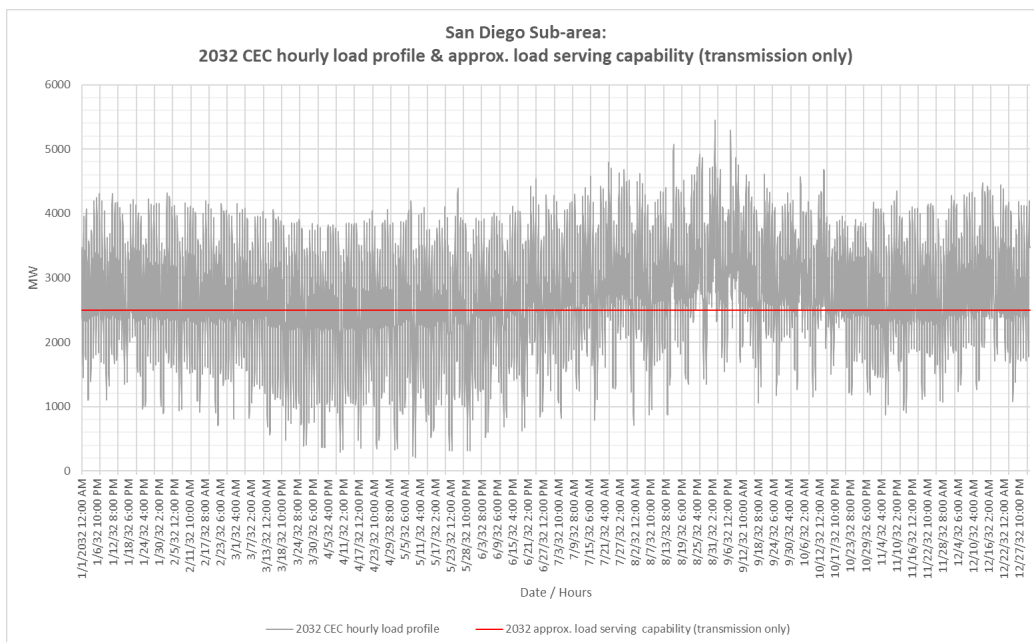
Figure J.3.2-87 San Diego LCR sub-area 2032 Forecast Hourly Profiles
