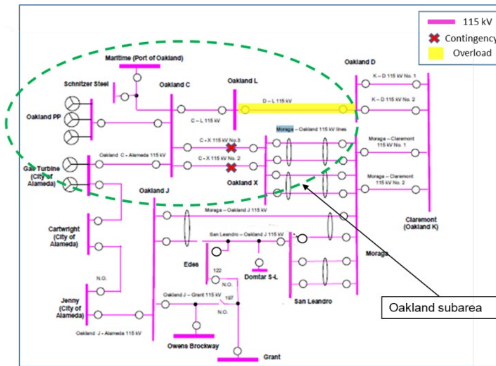
Figure J.3.2-30 Oakland LCR Sub-area
