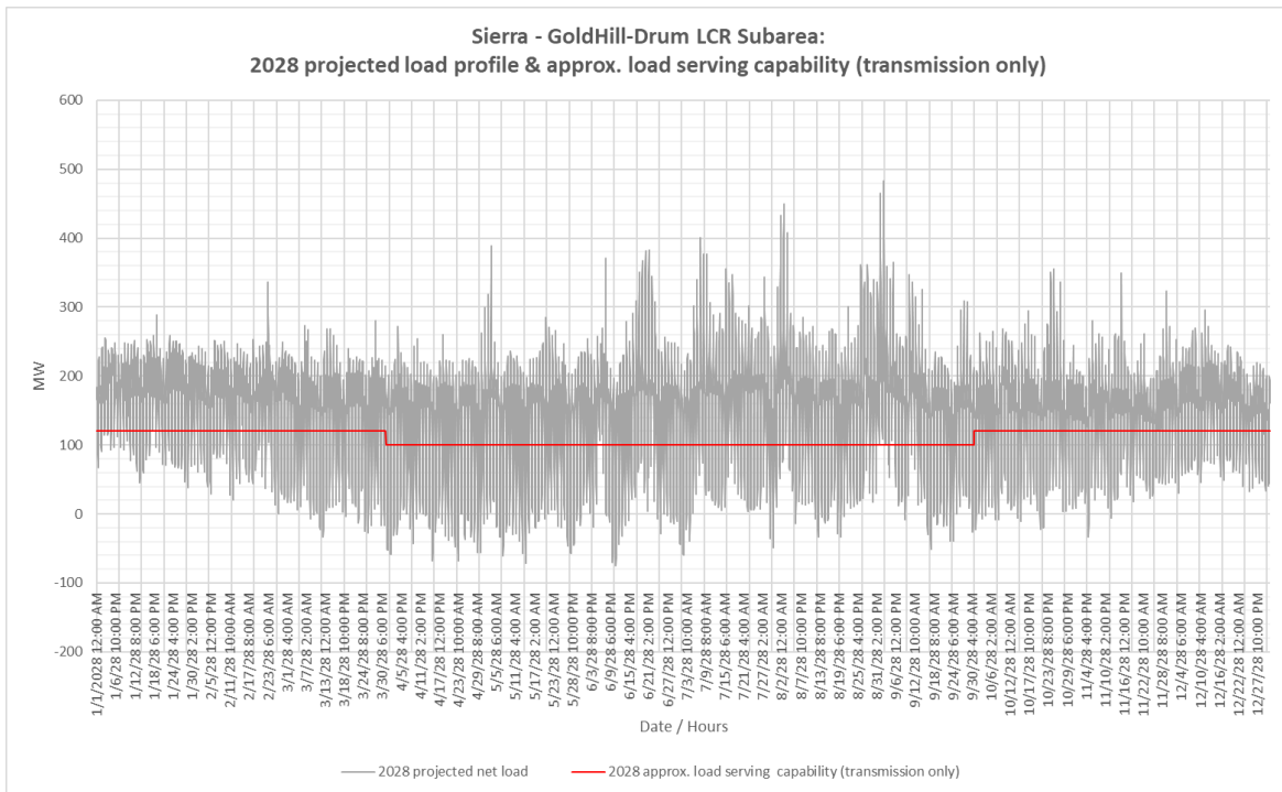
Figure 3.2-19 Gold Hill-Drum LCR Sub-area 2028 Forecast Hourly Profiles
