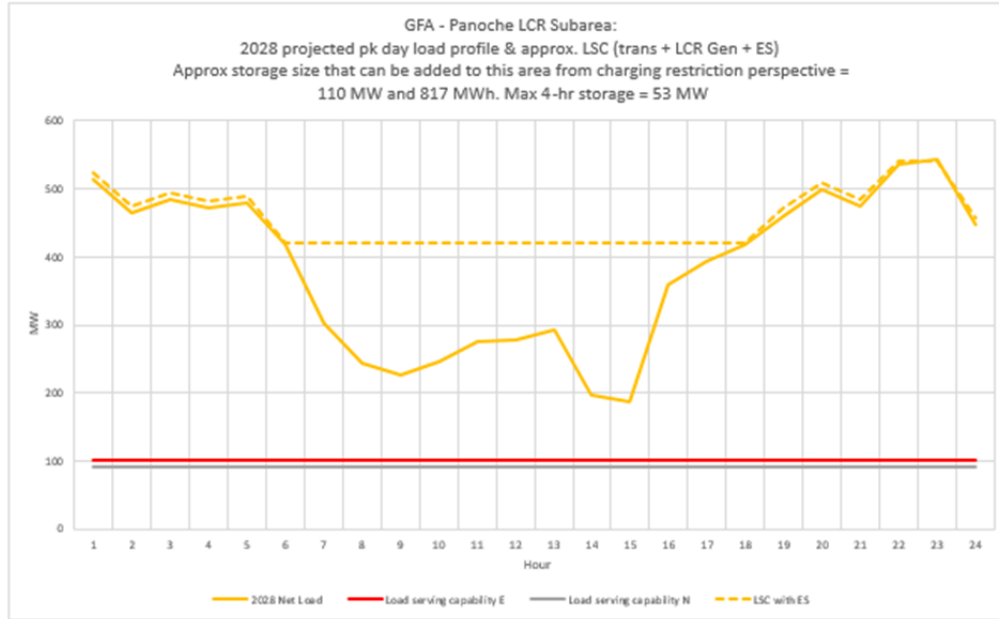
Figure 3.2-50 Panoche LCR Sub-area 2028 Forecast Hourly Profiles
