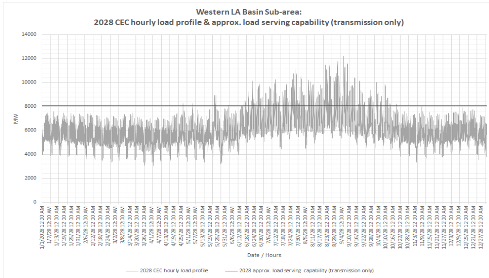
Figure 3.2-78 Western LA Basin LCR Sub-area 2028 Load Shape and Estimated Maximum Energy Storage Capacity and Energy Based on Charging Capability Under Critical Contingency
