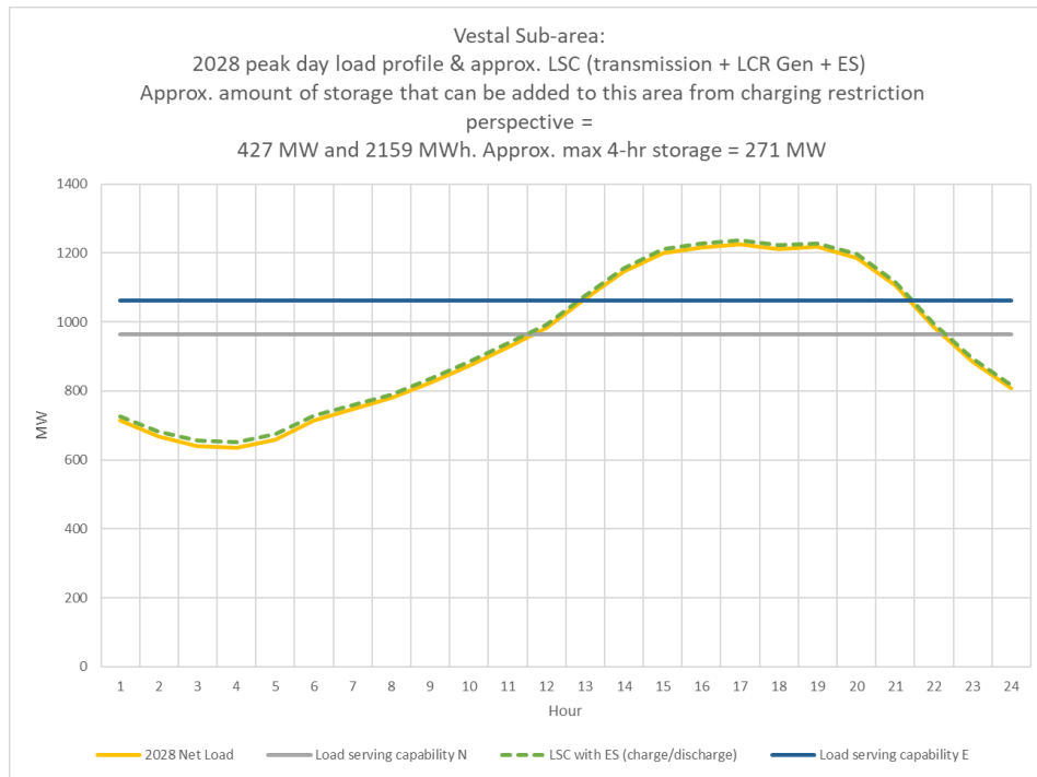
Figure 3.2-68 Vestal LCR Sub-area 2028 Load Shape and Estimated Maximum Energy Storage Capacity and Energy Based on Charging Capability Under Critical Contingency
