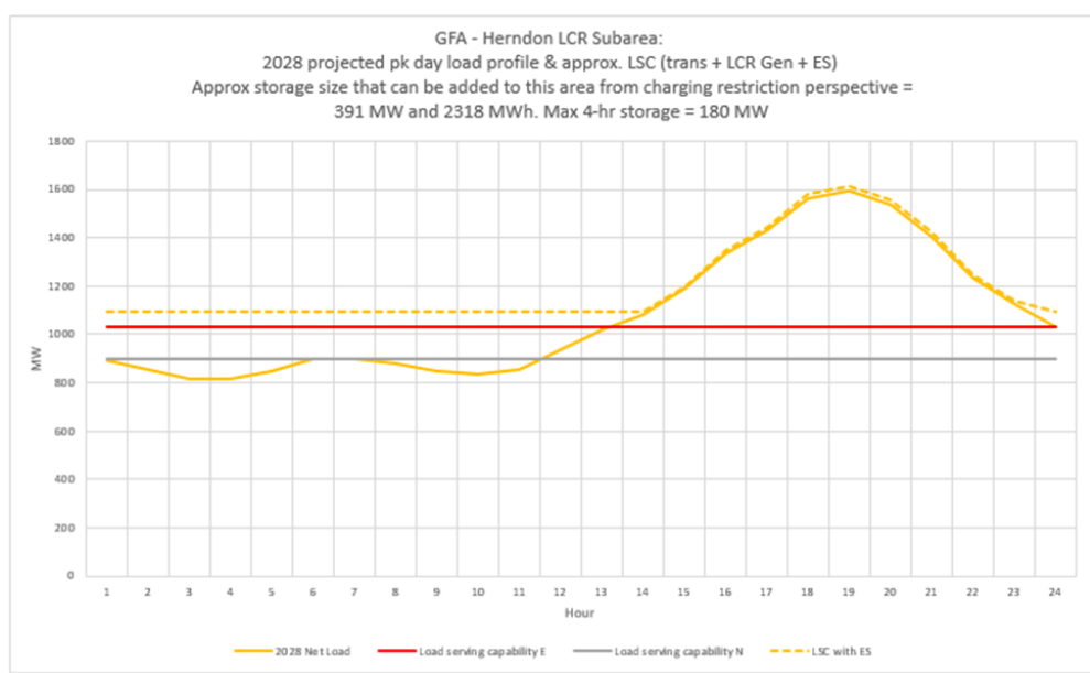
Figure 3.2-52 Herndon LCR Sub-area 2028 Peak Day Forecast Profiles
