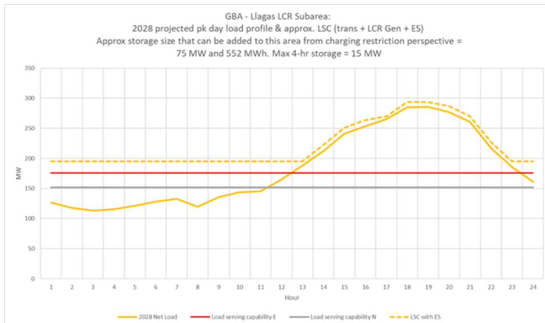
Figure 3.2-27 Llagas LCR Sub-area 2028 Peak Day Forecast Profiles
