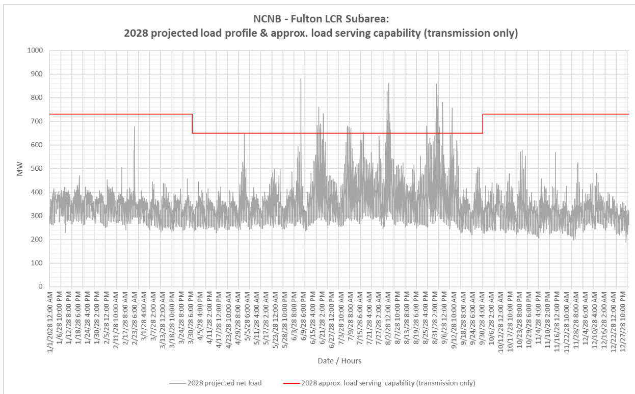
Figure 3.2-12 Fulton LCR Sub-area 2028 Forecast Hourly Profiles
