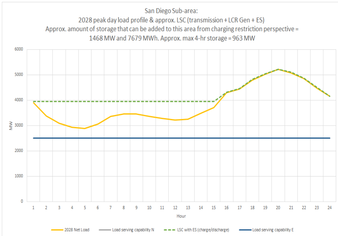
Figure 3.2-88 San Diego LCR Sub-area 2028 Load Shape and Estimated Maximum Energy Storage Capacity and Energy Based on Charging Capability Under Critical Contingency
