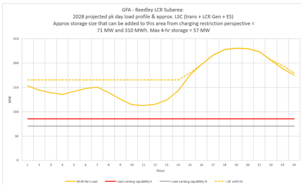
Figure 3.2-46 Reedley LCR Sub-area 2028 Peak Day Forecast Profiles
