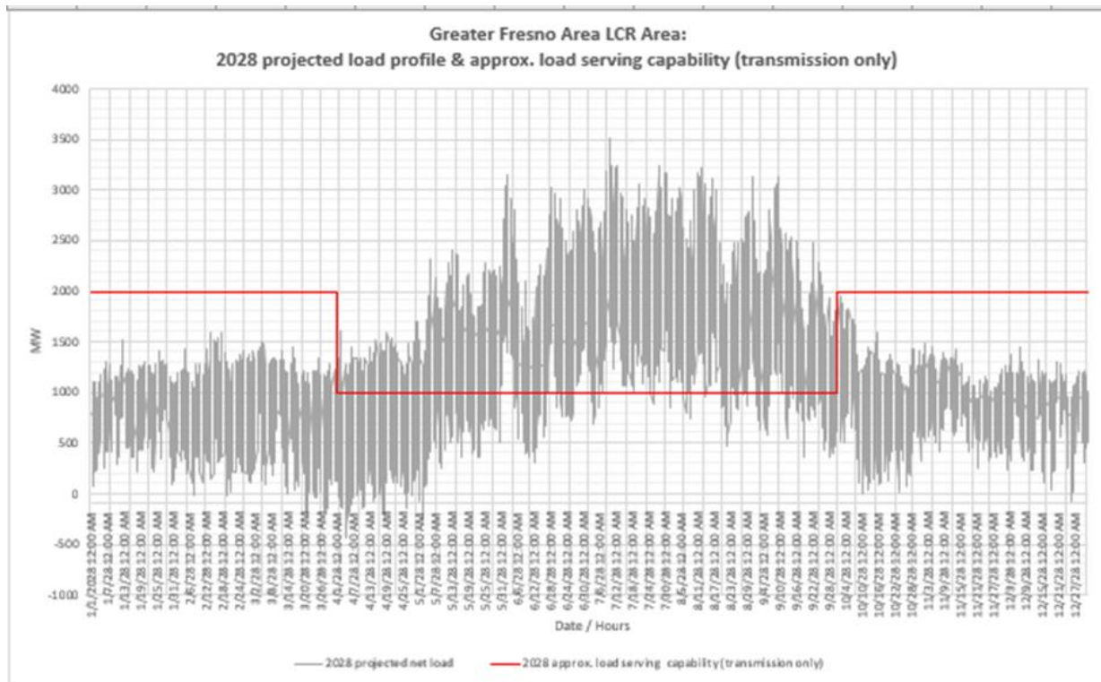
Figure 3.2-56 Fresno LCR Area 2028 Forecast Hourly Profiles
