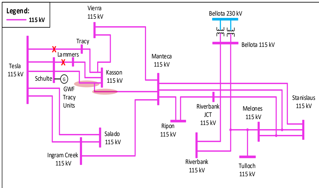
Figure 3.2-22 Tesla-Bellota LCR Sub-area
