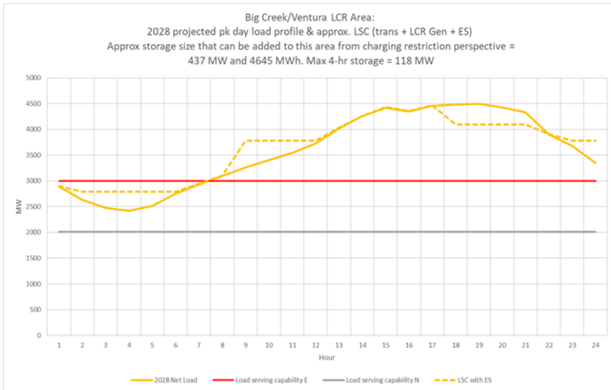
Figure 3.2-73 Big Creek/Ventura LCR area 2028 Load Shape and Estimated Maximum Energy Storage Capacity and Energy Based on Charging Capability Under Critical Contingency
