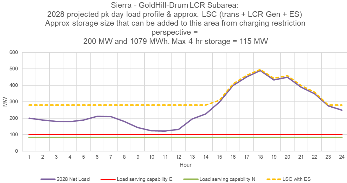
Figure 3.2-19 Gold Hill-Drum LCR Sub-area 2028 Forecast Hourly Profiles
