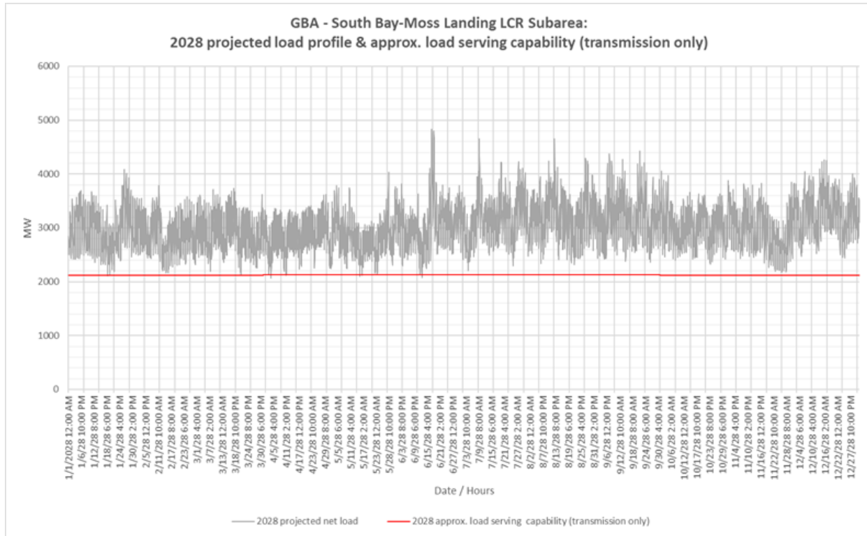
Figure 3.2-32 South Bay-Moss Landing LCR Sub-area 2028 Forecast Hourly Profiles
