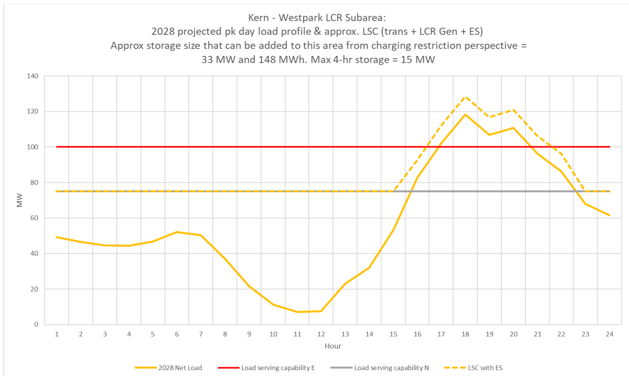
Figure 3.2-59 Westpark LCR Sub-area 2028 Forecast Hourly Profiles
