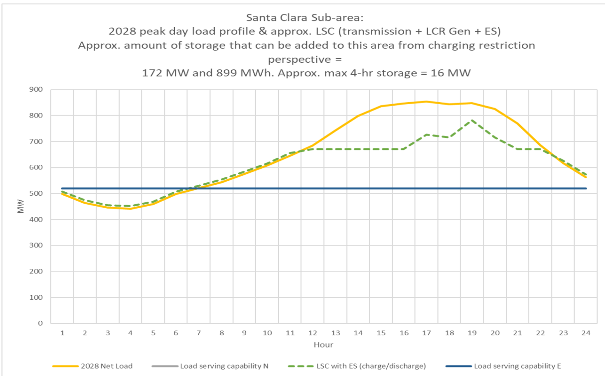
Figure 3.2-71 Santa Clara LCR Sub-area 2028 Load Shape and Estimated Maximum Energy Storage Capacity and Energy Based on Charging Capability Under Critical Contingency
