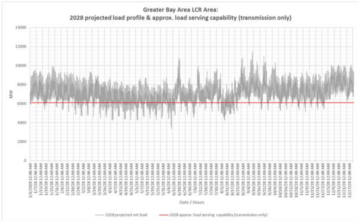
Figure 3.2-37 Bay Area LCR Area 2028 Forecast Hourly Profiles
