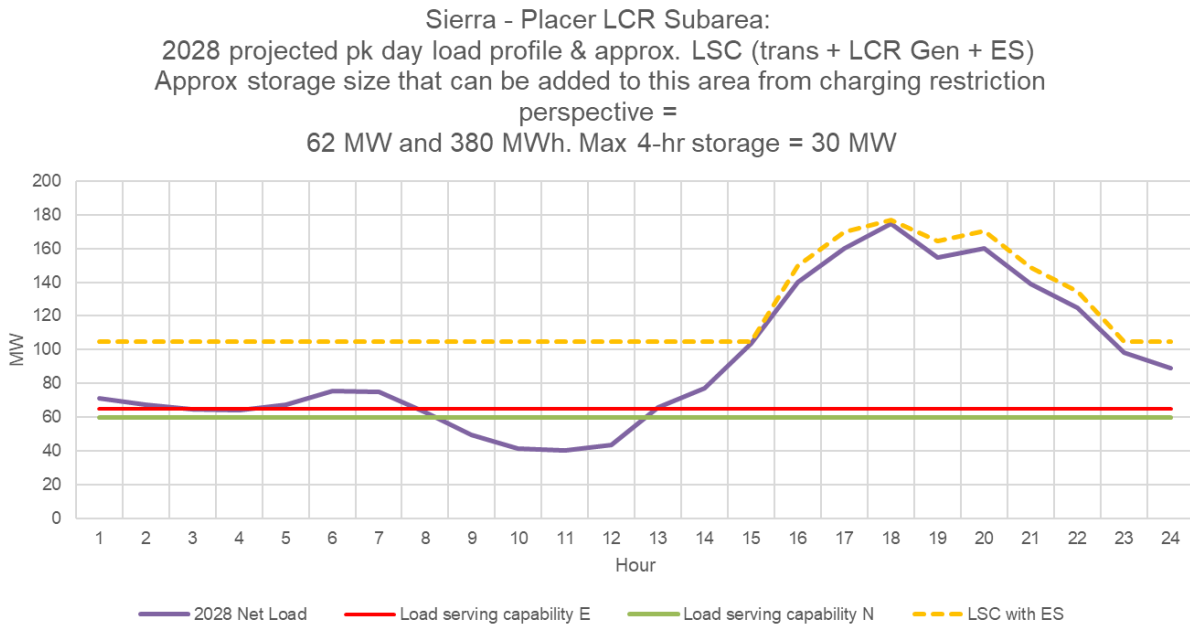
Figure 3.2-16 Placer LCR Sub-area 2028 Forecast Hourly Profiles
