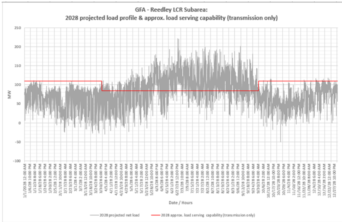
Figure 3.2-47 Reedley LCR Sub-area 2028 Forecast Hourly Profiles
