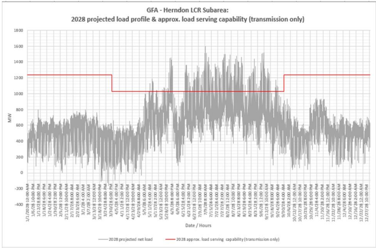
Figure 3.2-53 Herndon LCR Sub-area 2028 Forecast Hourly Profiles
