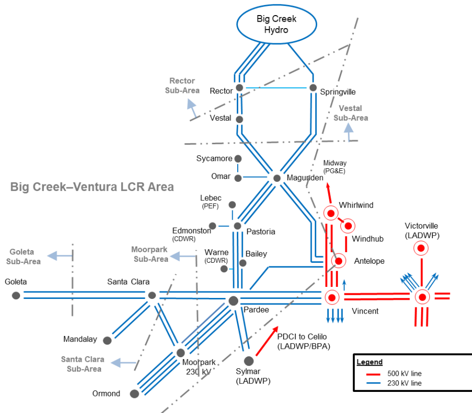
Figure 3.2-65 Big Creek/Ventura LCR Area
