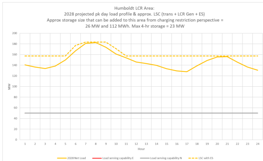
Figure 3.2-2 Humboldt 2028 Peak Day Forecast Profiles
