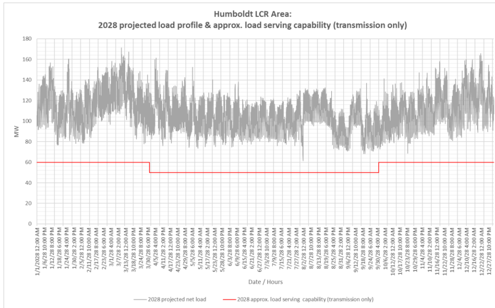
Figure 3.2-3 Humboldt 2028 Forecast Hourly Profile
