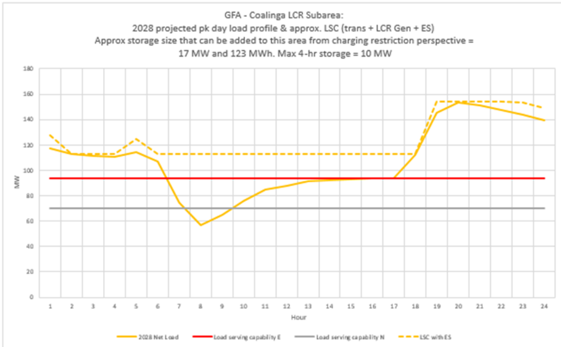
Figure 3.2-43 Coalinga LCR Sub-area 2028 Peak Day Forecast Profiles
