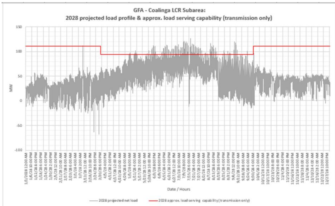
Figure 3.2-44 Coalinga LCR Sub-area 2028 Forecast Hourly Profiles
