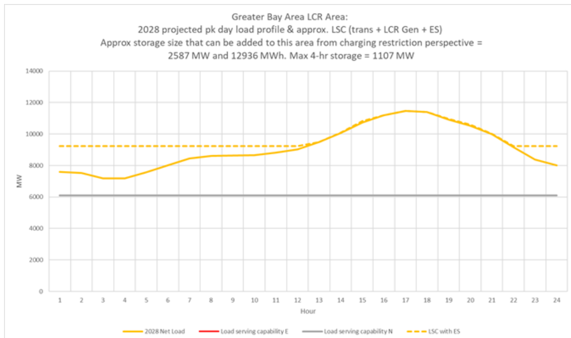
Figure 3.2-36 Bay Area LCR Area 2028 Peak Day Forecast Profiles
