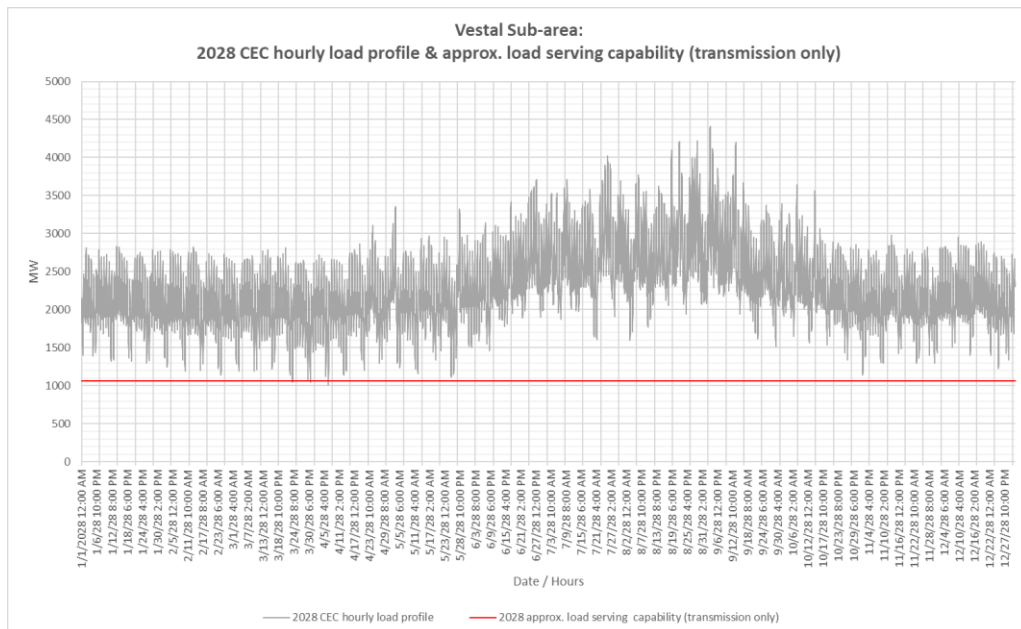
Figure 3.2-67 Vestal LCR Sub-area 2028 Annual Load Profile with Estimated Transmission Only Load Serving Capability
