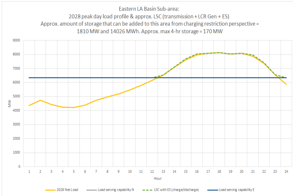
Figure 3.2-80 Eastern LA Basin LCR Sub-area 2028 Load Shape and Estimated Maximum Energy Storage Capacity and Energy Based on Charging Capability Under Critical Contingency
