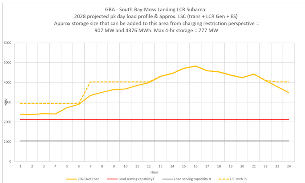
Figure 3.2-31 South Bay-Moss Landing LCR Sub-area 2028 Peak Day Forecast Profiles
