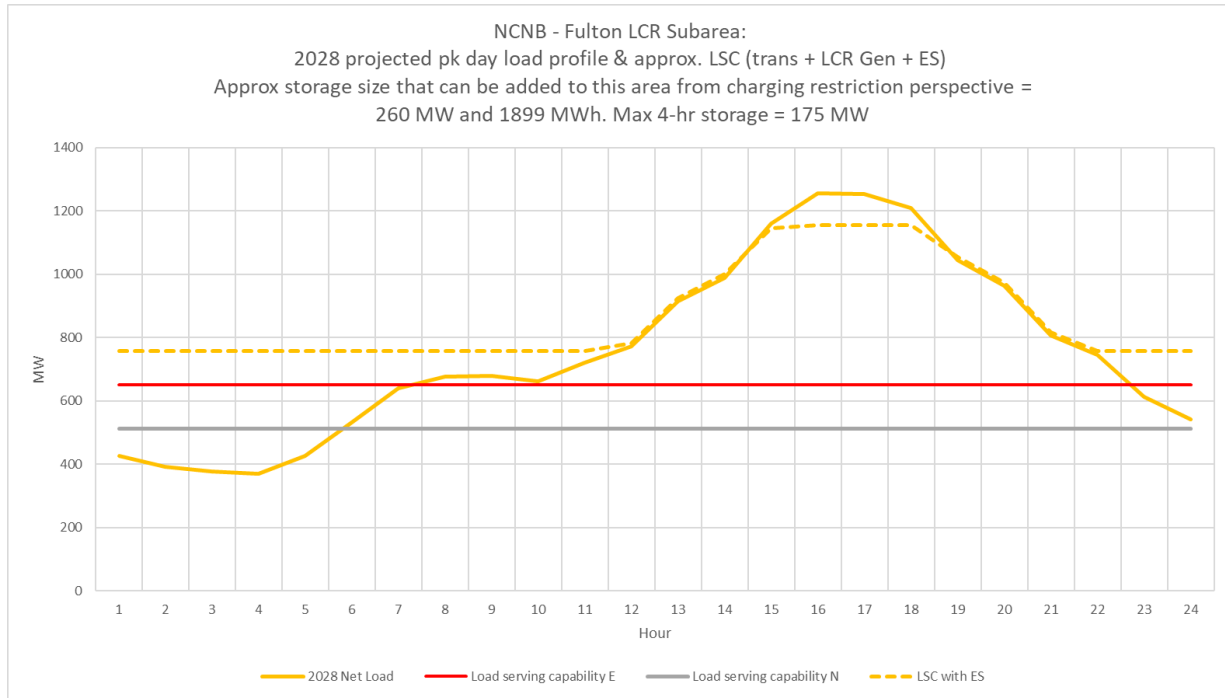
Figure 3.2-12 Fulton LCR Sub-area 2028 Forecast Hourly Profiles
