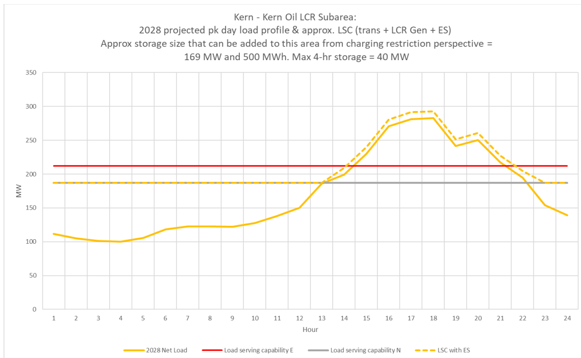
Figure 3.2-61 Kern Oil LCR Sub-area 2028 Forecast Hourly Profiles
