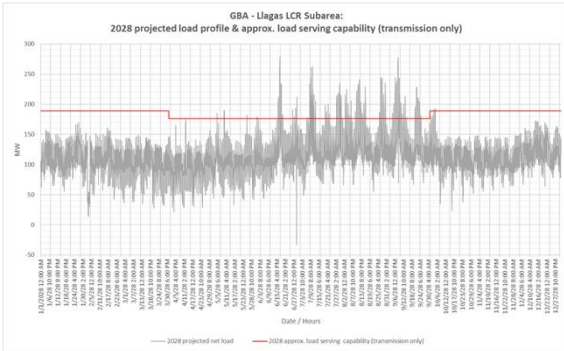
Figure 3.2-28 Llagas LCR Sub-area 2028 Forecast Hourly Profiles
