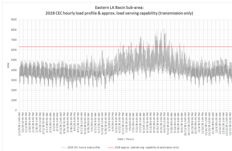
Figure 3.2-79 Eastern LA Basin LCR Sub-area 2028 Annual Load Profile with Estimated Transmission Load Serving Capability Only
