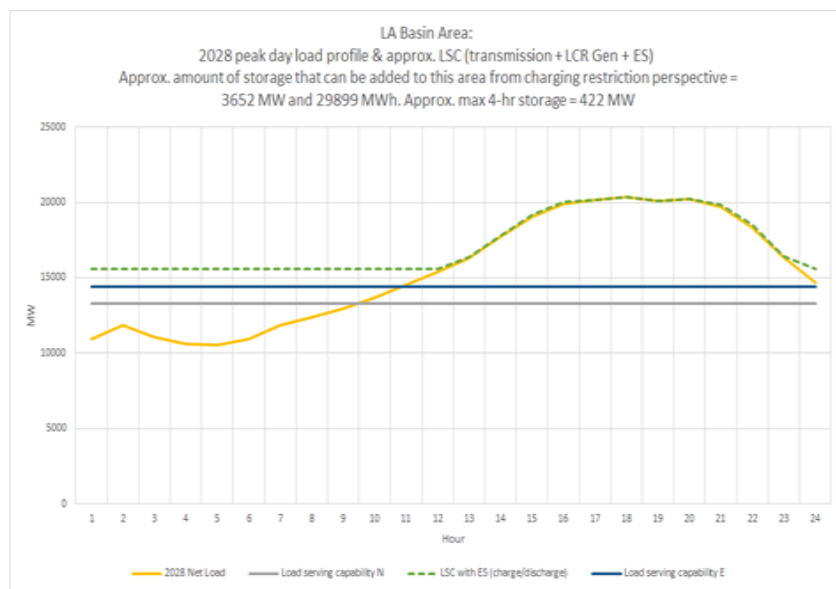
Figure 3.2-82 LA Basin LCR Area 2028 Load Shape and Estimated Maximum Energy Storage Capacity and Energy Based on Charging Capability Under Critical Contingency
