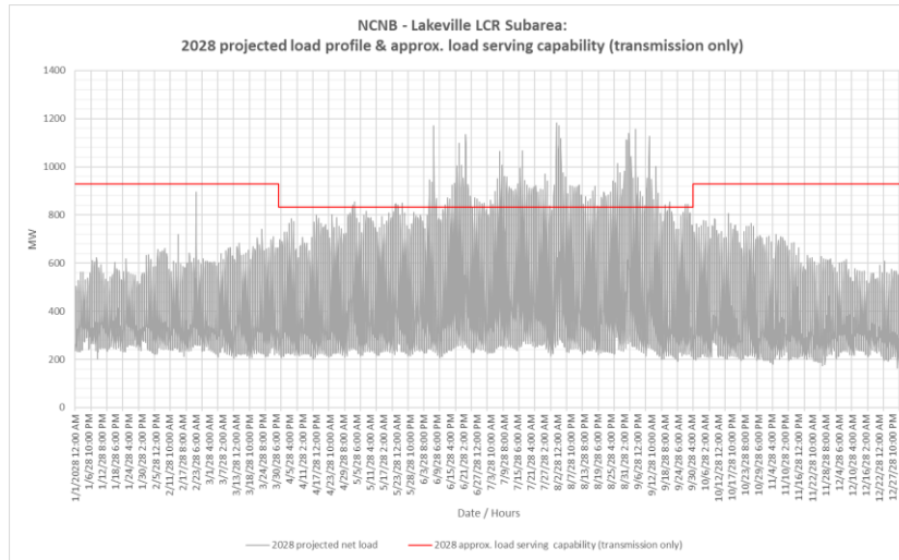
Figure 3.2-6 North Coast and North Bay 2028 Forecast Hourly Profile
