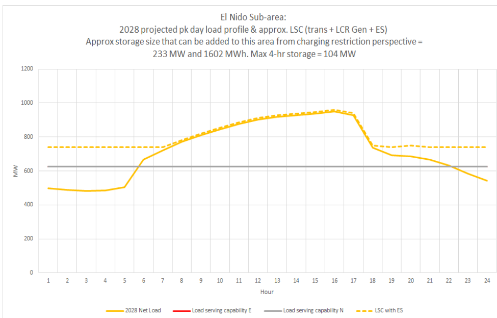
Figure 3.2-76 EI Nido LCR Sub-area 2028 Load Shape and Estimated Maximum Energy Storage Capacity and Energy Based on Charging Capability Under Critical Contingency
