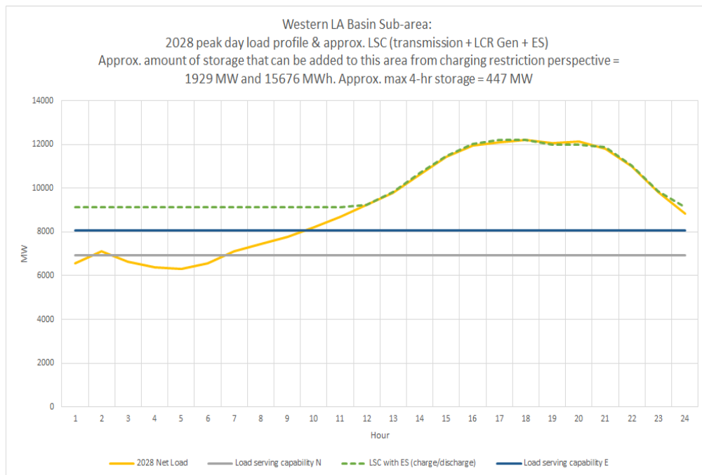
Figure 3.2-78 Western LA Basin LCR Sub-area 2028 Load Shape and Estimated Maximum Energy Storage Capacity and Energy Based on Charging Capability Under Critical Contingency
