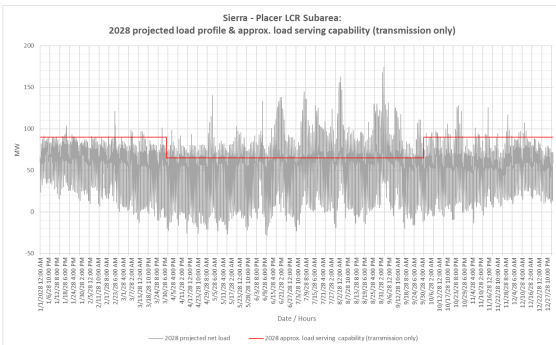
Figure 3.2-16 Placer LCR Sub-area 2028 Forecast Hourly Profiles
