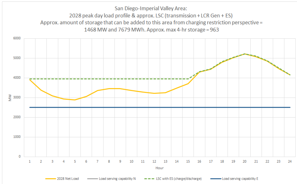
Figure 3.2-90 San Diego-Imperial Valley LCR Area 2028 Load Shape and Estimated Maximum Energy Storage Capacity and Energy Based on Charging Capability Under Critical Contingency
