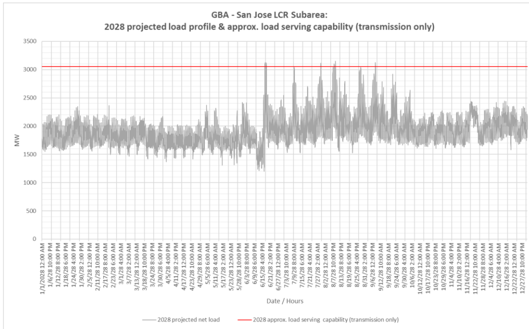
Figure 3.2-30 San Jose LCR Sub-area 2028 Forecast Hourly Profiles
