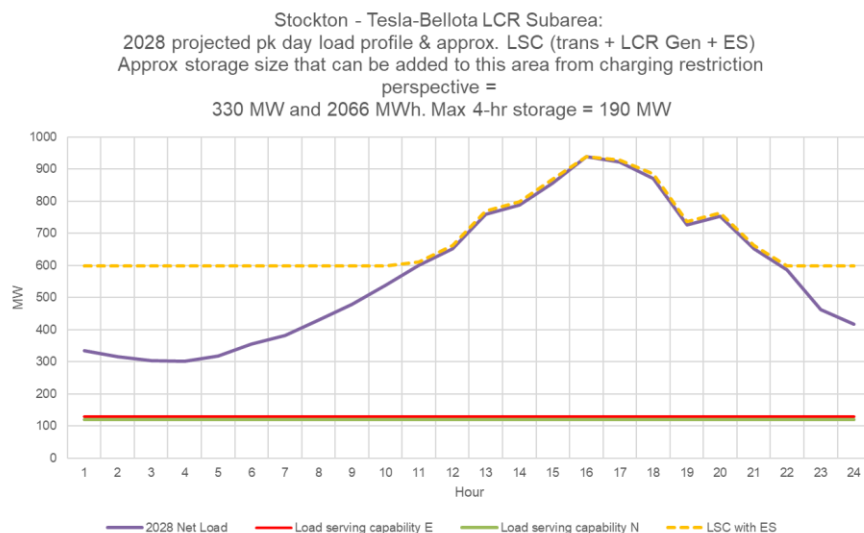
Figure 3.2-23 Tesla-Bellota LCR Sub-area 2028 Peak Day Forecast Profiles
