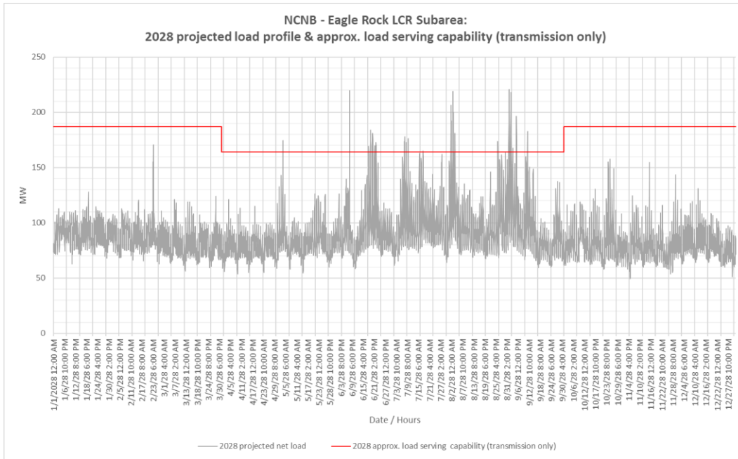
Figure 3.2-9 Eagle Rock LCR Sub-area 2028 Forecast Hourly Profiles
