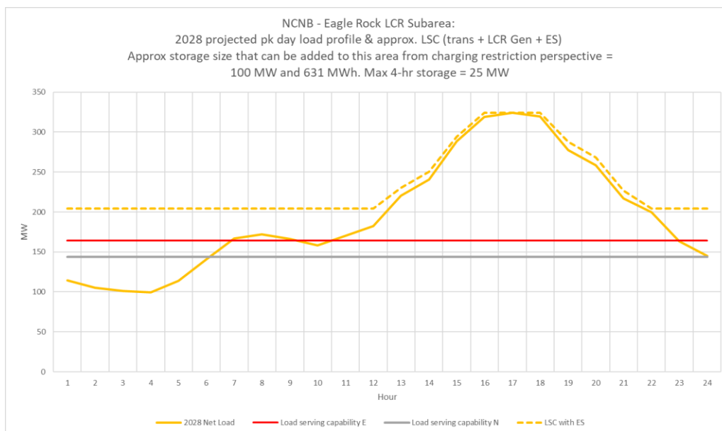
Figure 3.2-8 Eagle Rock LCR Sub-area 2028 Peak Day Forecast Profiles
