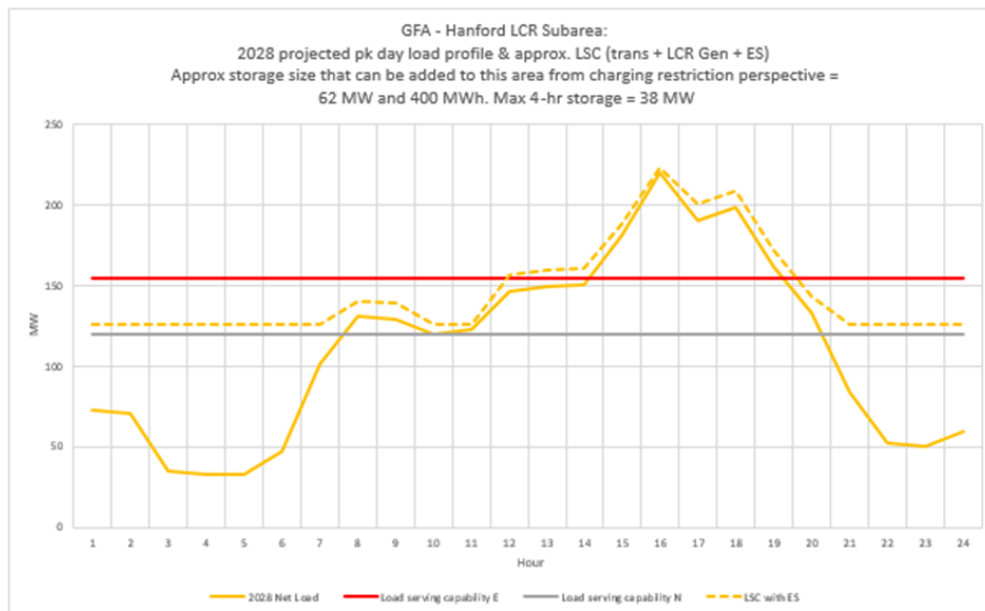
Figure 3.2-40 Hanford LCR Sub-area 2028 Peak Day Forecast Profiles
