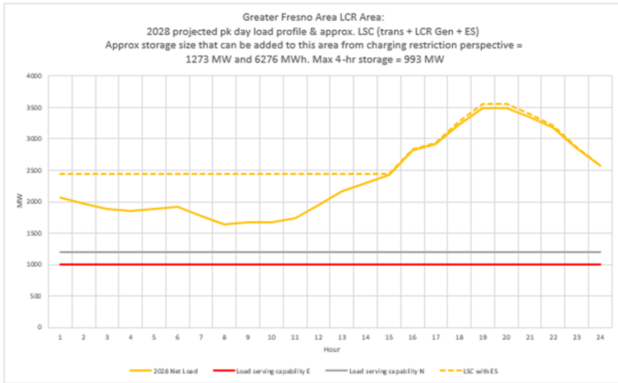
Figure 3.2-55 Fresno LCR Area 2028 Peak Day Forecast Profiles
