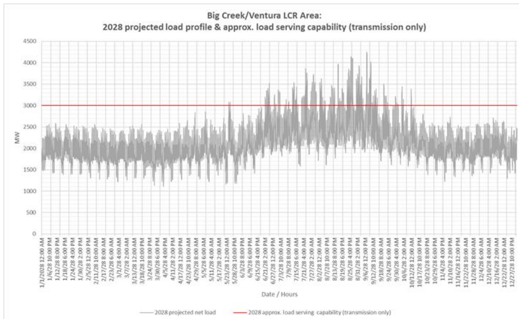
Figure 3.2-72 Big Creek/Ventura LCR area 2028 Annual Load Profile with Estimated Transmission Only Load Serving Capability
