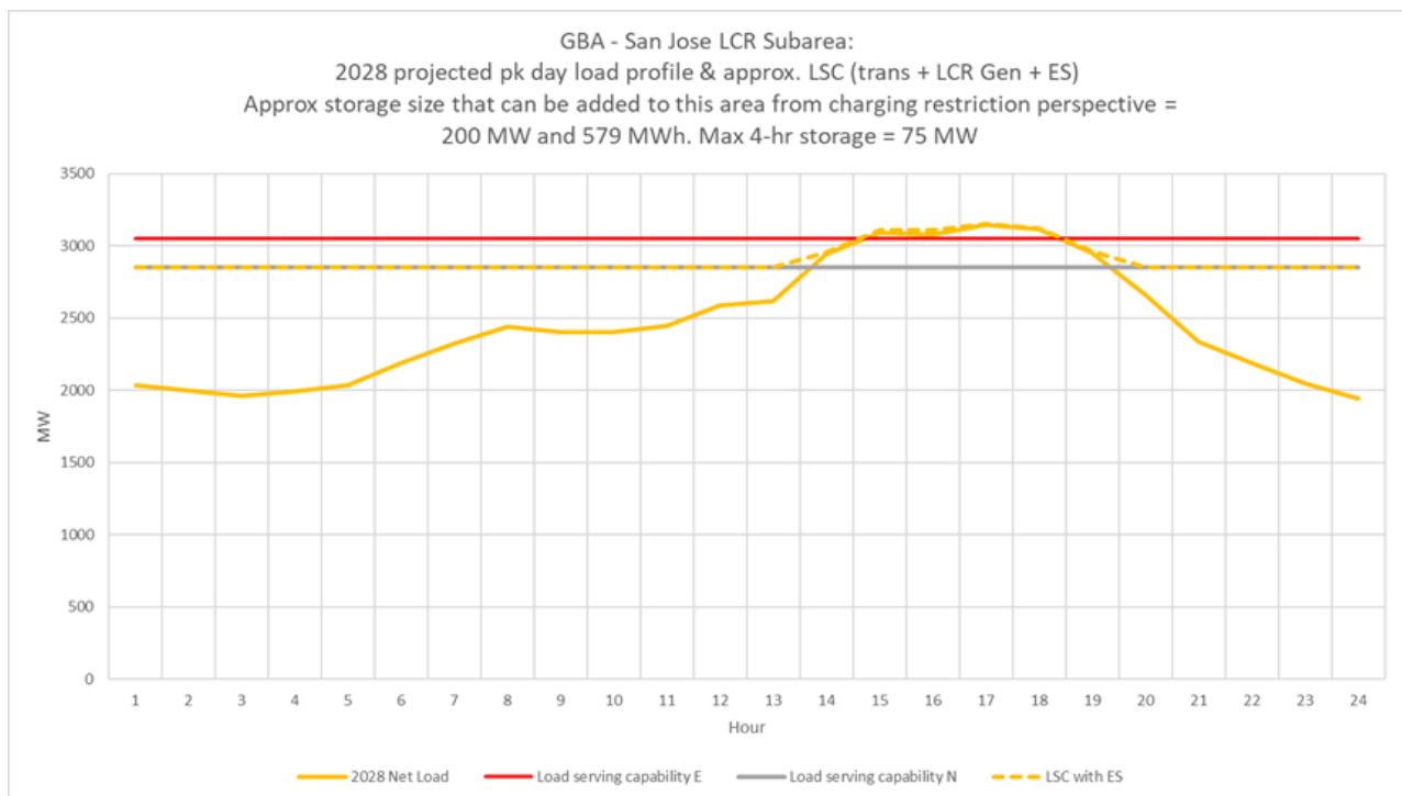
Figure 3.2-29 San Jose LCR Sub-area 2028 Peak Day Forecast Profiles
