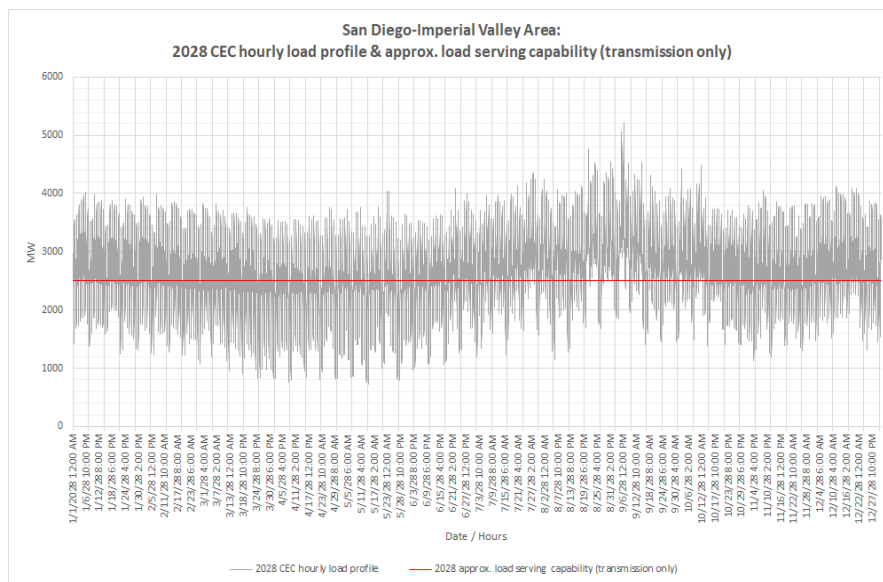
Figure 3.2-89 San Diego-Imperial Valley LCR Area 2028 Annual Load Profile with Estimated Transmission Load Serving Capability Only
