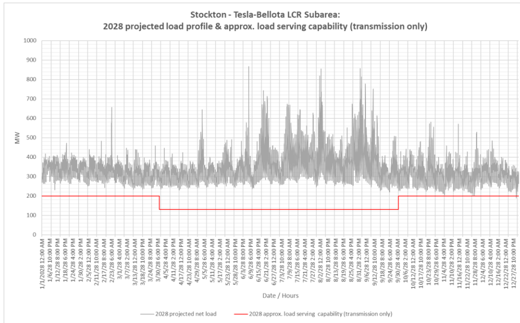
Figure 3.2-24 Tesla-Bellota LCR Sub-area 2028 Forecast Hourly Profile
