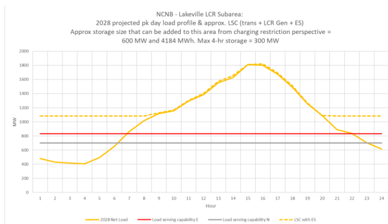
Figure 3.2-5 North Coast and North Bay 2028 Peak Day Forecast Profiles
