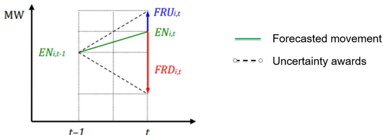
Figure 8: Forecasted movement and uncertainty awards
